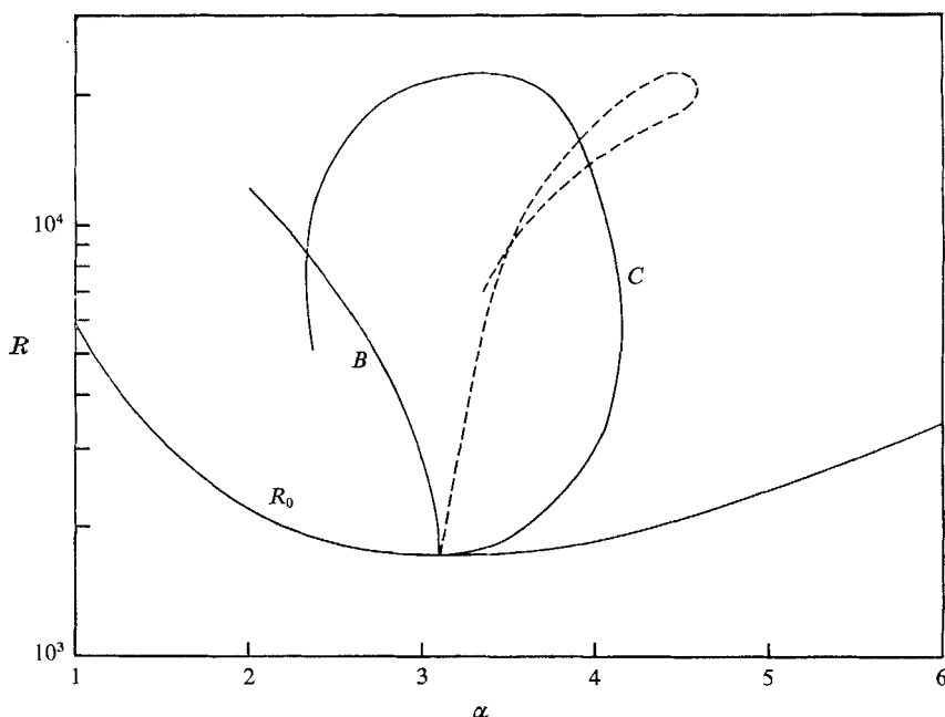
FIGURE 1. Stability region of convection rolls. The zigzag instability and the cross-roll instability produce the stability boundaries B and C , respectively. The dashed line denotes the value of the wave-number \tilde{\alpha} of the marginal cross-roll disturbances along curve C .
