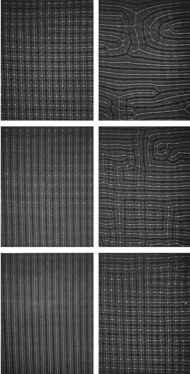
FIGURE 12. Cross-roll instability at R = 21 \times 10^8 , d = 1 cm, \alpha = 2\pi/1.5 . Time intervals between subsequent photographs are 4, 8, 4, 10, and 24 min, respectively.
