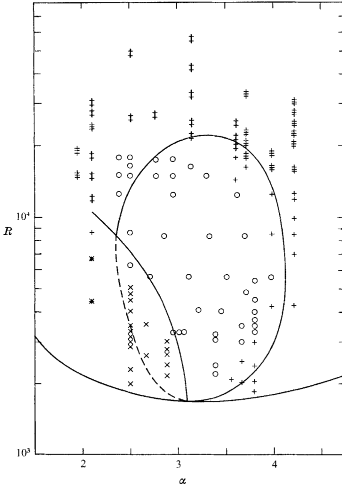
FIGURE 6. Experimental results. \circ , stable rolls; \times , zigzag instability; + , cross-roll instability leading to rolls; \# , cross-roll instability leading to bimodal convection; \oplus , cross-roll instability inducing transient rolls with subsequent local processes. The curves correspond to the theoretical results shown in figure 1.
